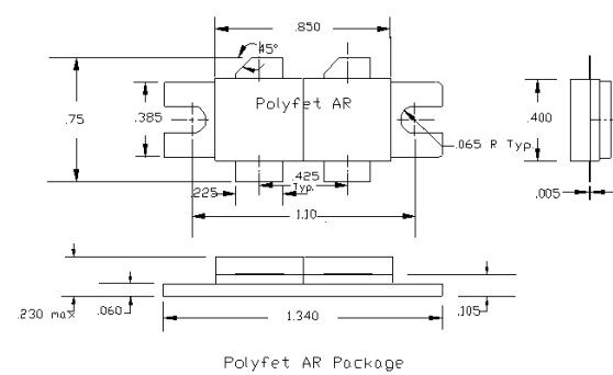
PACKAGE DIMENSIONS IN INCHES
